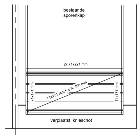
dakplan
