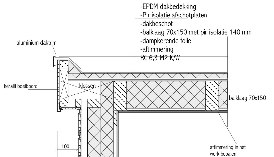
detail 3
