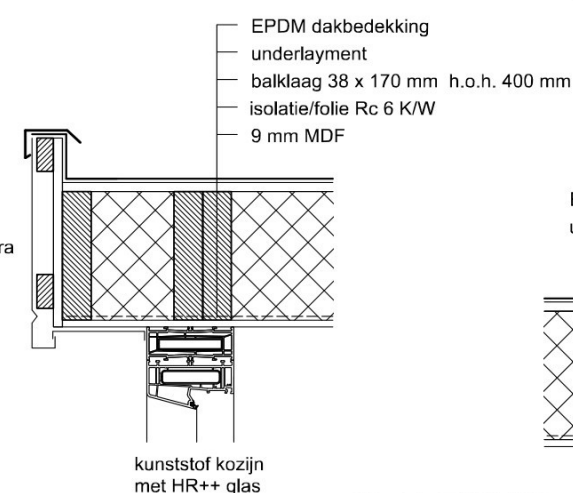
PRINCIPEDetails schaal 1:10
