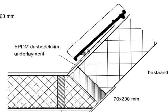
PRINCIPEDetails schaal 1:10
