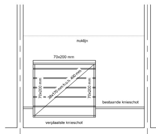
dakplan
